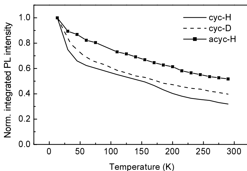
Figure 2.7 Temperature dependence of the integrated 1.54 \mu\text{m} PL intensity of the \text{Er}^{3+} complexes in KBr (pump power 100 mW, excitation wavelength 488 nm).
