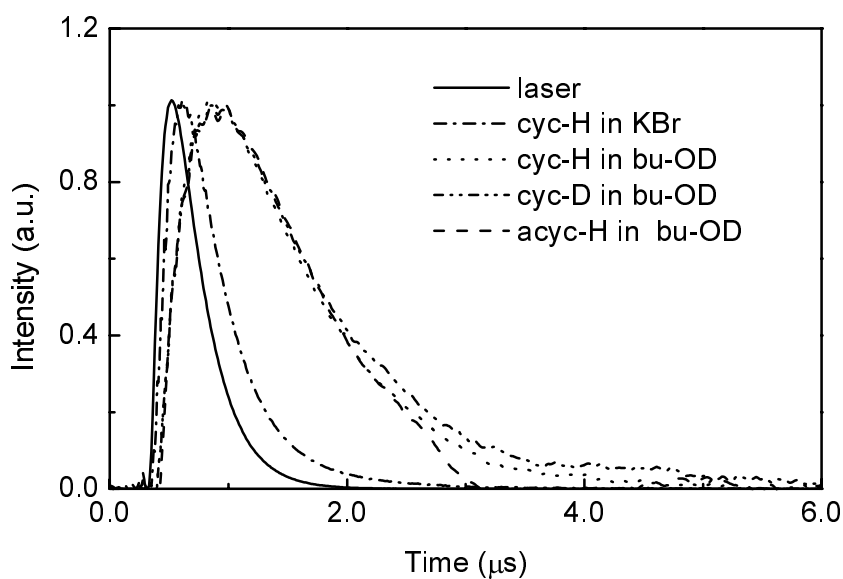
Figure 2.6 Room temperature decay measurements for the Er-doped organic complexes in KBr and butanol-OD, excited at 337 nm at a pulse energy of 20 \mu J.
