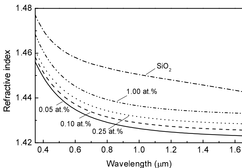
Figure 6.3 Refractive index as a function of wavelength for spin-coated films doped with different Er concentrations (before annealing). Data for thermally grown \text{SiO}_2 are also shown. 15
