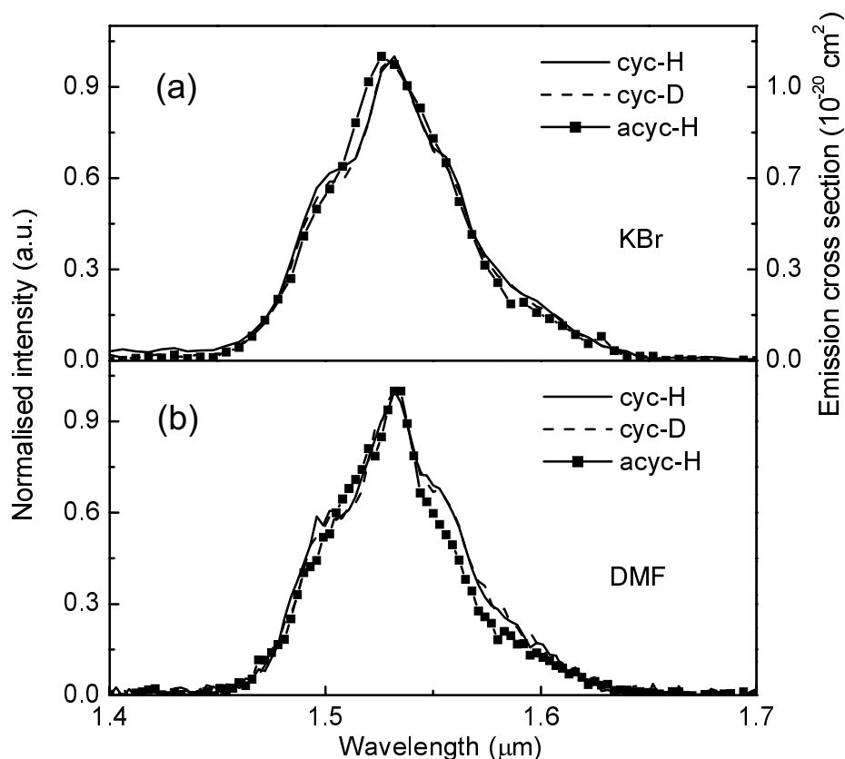
Figure 2.3 Normalised room temperature PL spectra of \text{Er}^{3+} complexes in (a) KBr tablets and (b) DMF, at a pump wavelength of 488 nm (power 100 mW).
