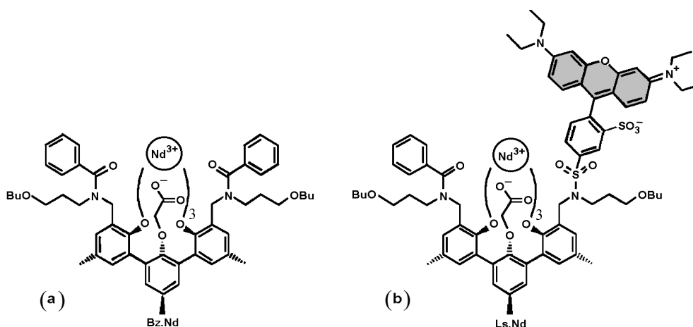
Figure 3.2 Schematic picture of (a) benzoyl- \text{Nd}^{3+} complex (Bz.Nd) and (b) lissamine functionalised \text{Nd}^{3+} complex (Ls.Nd).
