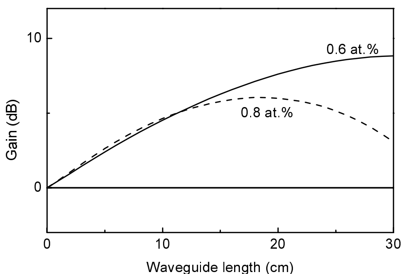
Figure 7.8 Total gain as a function of waveguide length for an Er-doped colloid/polymer composite waveguide amplifier pumped at 1.48\ \mu\text{m} . Data are shown for Er concentrations in the colloid of 0.6 at.% (solid line) and 0.8 at.% (dashed line), at an input power of 20 mW.
