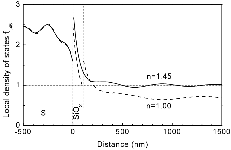
Figure 8.2 Polarization- and angle-averaged optical local DOS, for a 100 nm thick \text{SiO}_2 layer ( n = 1.45 ). The layer is sandwiched between a Si substrate ( n = 3.45 ) and an ambient with n = 1.00 (dashed line) or n = 1.45 (solid line). All calculations were done for a wavelength of 1.54 \mu\text{m} .
