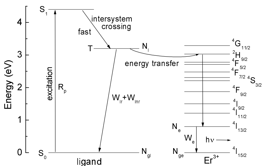
Figure 2.1 Schematic diagram of the ligand- \text{Er}^{3+} system. The complex is first excited from the singlet S_0 ground state to the singlet S_1 state (exact position not known, but higher than 3.2 eV), followed by fast relaxation to the triplet T state. From there, energy transfer to the \text{Er}^{3+} 4f levels may take place. From these levels, rapid relaxation to the ^4I_{13/2} takes place. Finally the \text{Er}^{3+} may decay to the ^4I_{15/2} ground manifold by emission of a 1.54 \mu\text{m} photon. The various symbols are discussed in the text.
