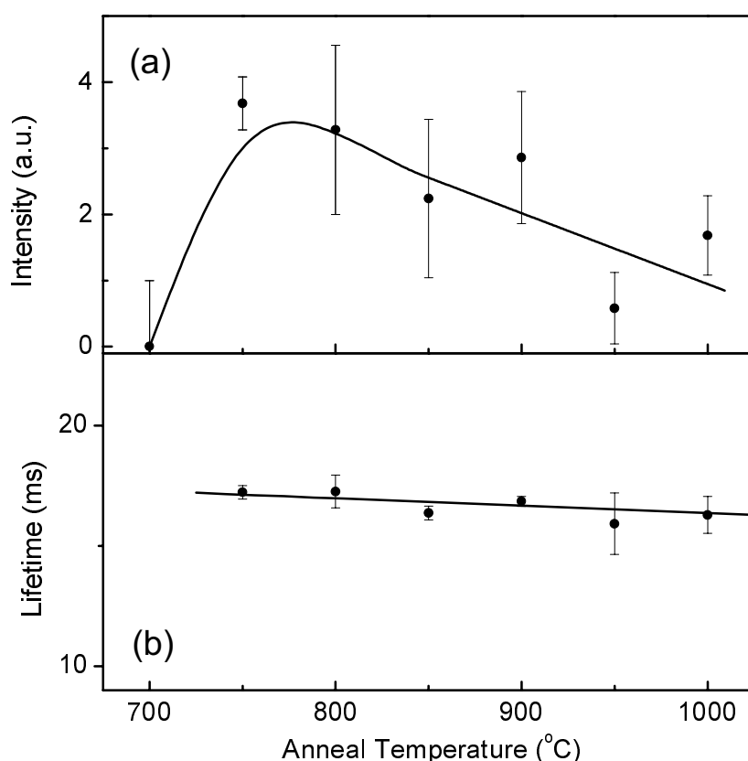
Figure 7.3 (a) Average peak photoluminescence intensity at 1.53\ \mu\text{m} as a function of anneal temperature for Er-implanted silica spheres (0.2 at.%). Pump wavelength 488 nm, pump power 50 mW. The large error bars are due to the large variation in colloid coverage over the surface. (b) Luminescence lifetime of Er-implanted silica spheres (0.2 at.%) as a function of anneal temperature.
