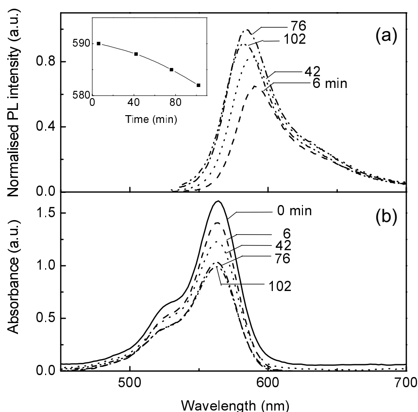
Figure 4.2 Luminescence (a) and absorption (b) spectra of the lissamine sensitizer for different illumination times. The excitation wavelength was 488 nm at a pump power of 1 W in a 5 mm spot. The inset shows the peak position in nm as a function of the illumination time.
