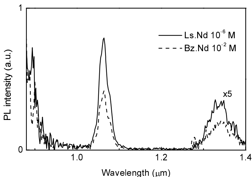
Figure 3.4 Photoluminescence spectra of Ls.Nd ( 10^{-6} M) and Bz. Nd ( 10^{-2} M) in DMSO-d 6 solutions. The excitation wavelength is 515 nm, at a pump power of 60 mW. Note that around 1340 nm the spectra are multiplied by a factor 5.
